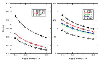
Fig. 4: (a) Discharge time vs. Supply Voltage for RV, SE, and HV cells. (b) Discharge time vs. Supply Voltage for RV, OA, LE, SE, and HV cells.
