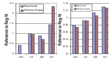
Fig. 5: (a) Reference to Reg-Vt for Nominal and Worst-Case conditions across OA, LE, SE, and HV cells. (b) Reference to Reg-Vt for Nominal and Worst-Case conditions across OA, LE, SE, and HV cells.
