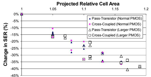
Figure 11: Summary of tradeoff between cell-area and SER
