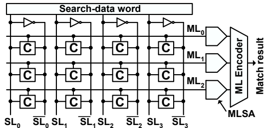
Figure 1: Organization of a Content Addressable Memory
