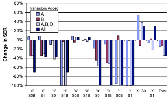
Figure 9: Breakdown in the reduction in the SER of various pass-transistor cells
