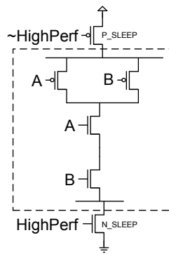
Fig. 1. Supply Gating
