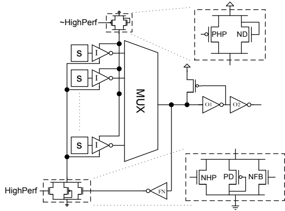
Fig. 8. Novel LUT
